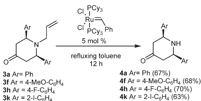
Scheme 2. Deprotection of N -allyl-4-piperidones using Grubbs catalyst.
