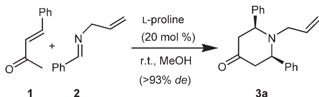
Scheme 1. Imino-Diels–Alder reaction catalyzed by L-proline.
