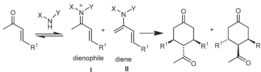
Figure 2. Amine-catalyzed Diels–Alder dimerization reactions.
