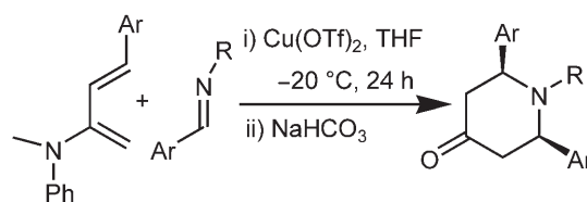
Figure 1. Preparation of meso -2,6-disubstituted-4-piperidones using a Lewis acid as catalyst.
