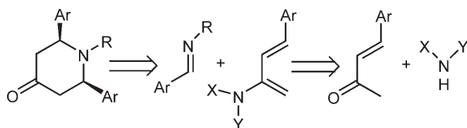
Figure 3. Retrosynthetic analysis for the synthesis of meso -2,6-diaryl-4-piperidones.
