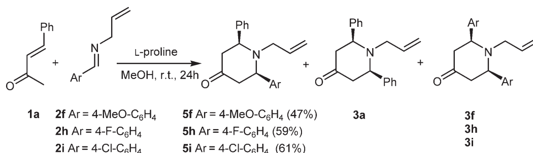
Scheme 3. Preparation of unsymmetrical 2,6-disubstituted-4-piperidones 5 .
