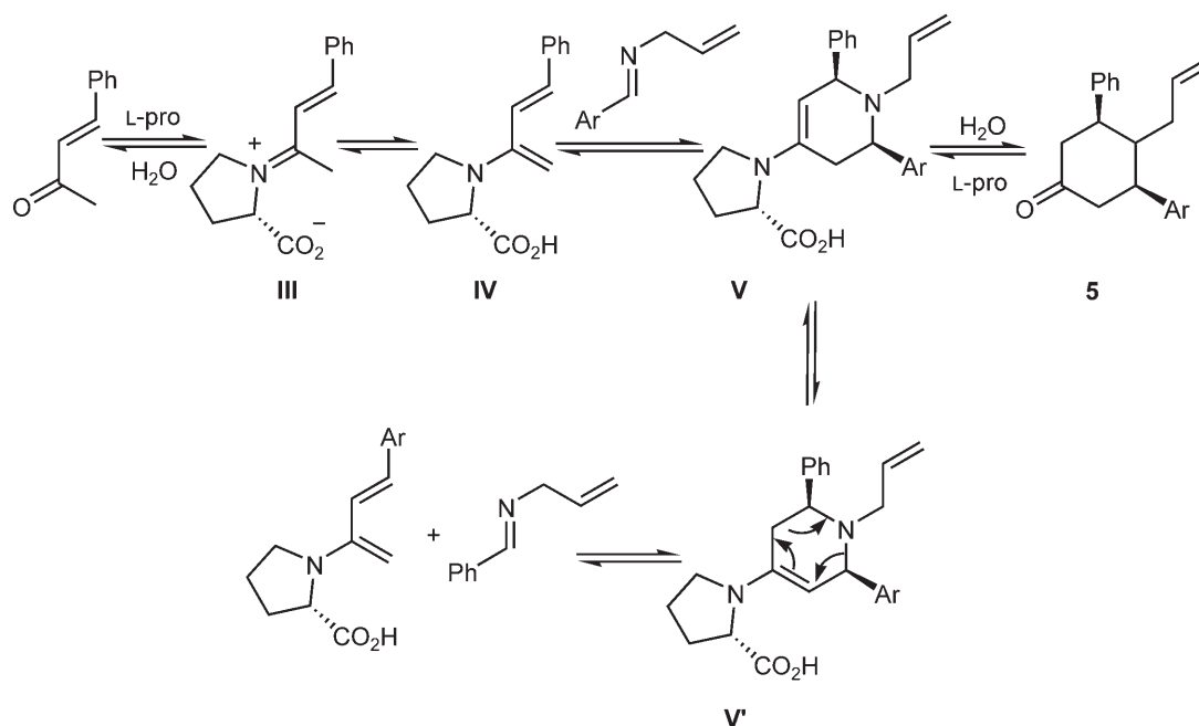
Scheme 4. A putative pathway for the proline-catalyzed imino-Diels–Alder reaction leading to unsymmetrical 2,6-disubstituted-4-piperidones 5 .
